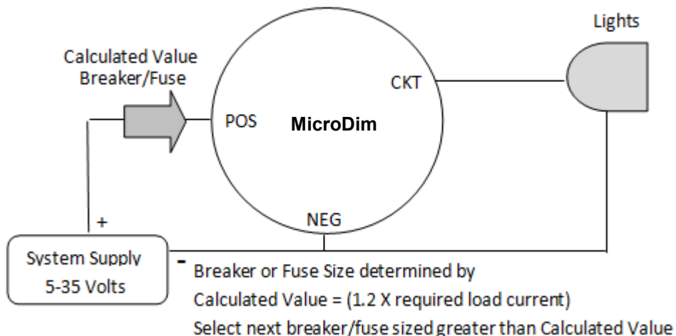
Wiring Diagram 9100-001-N MicroDim
